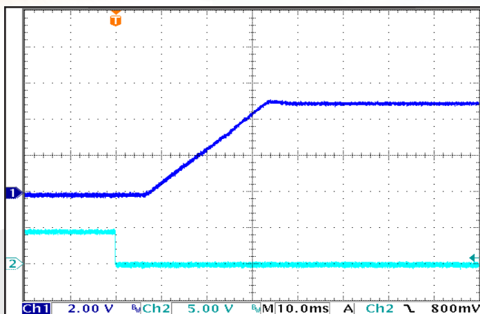
Figure 7: Typical Startup Waveform, input voltage pre-applied. Ch 1: V_{out} (2 V/div); Ch 2: ON/OFF Pin (5 V/div).
