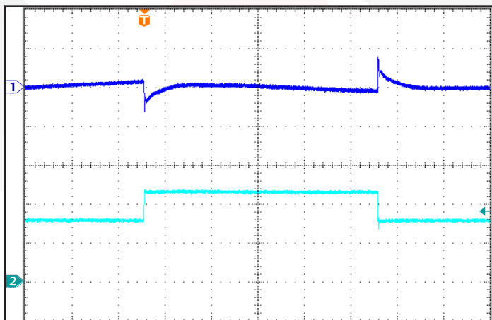
Figure 11: Output Voltage Response to Step-Change in Load Current, (50%-75%-50% of I_{out(max)} ; dI/dt = 5 A/ \mu s). Load capacitance: 1 \mu F ceramic and 100 \mu F electrolytic capacitors. Ch 1: \Delta V_{out} (0.5 V/div); Ch 2: I_{out} (20 A/div).
