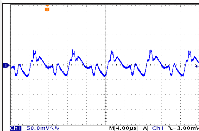
Figure 10: Output Voltage Ripple, V_{out} , at nominal input voltage and rated load current (50 mV/div). Load capacitance: 1 \mu F ceramic and 100 \mu F electrolytic capacitors. Bandwidth: 20 MHz. See Figure 13.
