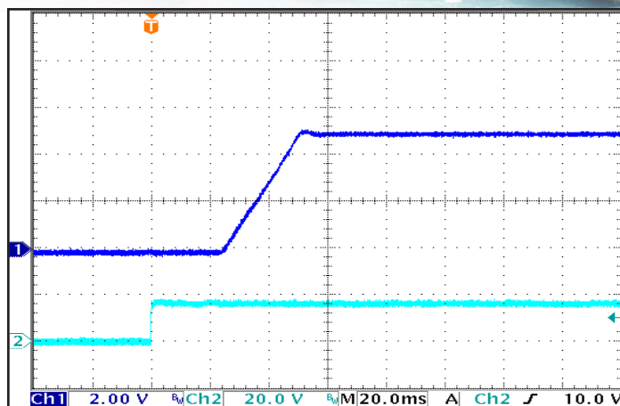
Figure 8: Turn-On Transient, at full resistive load and zero output capacitance, initiated by V_{in} . Ch 1: V_{out} (2 V/div); Ch 2: V_{in} (20 V/div).
