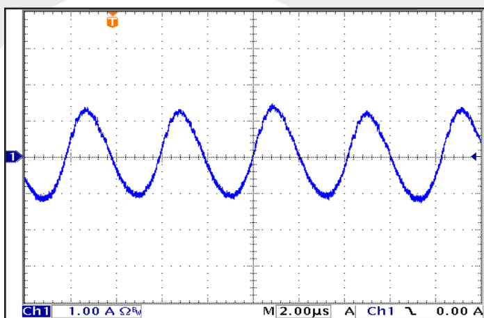
Figure 9: Input Terminal Current Ripple, i_c , at full rated output current and nominal input voltage with a 470 \mu F electrolytic capacitor (1 A/div). Bandwidth: 20 MHz. See Figure 13.
