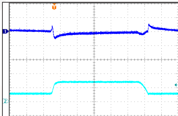
Figure 12: Output Voltage Response to Step-Change in Input Voltage, (250 V/ms). Load capacitance: 1 \mu F ceramic and 100 \mu F electrolytic capacitors. Ch 1: \Delta V_{out} (1 V/div); Ch 2: V_{in} (20 V/div).
